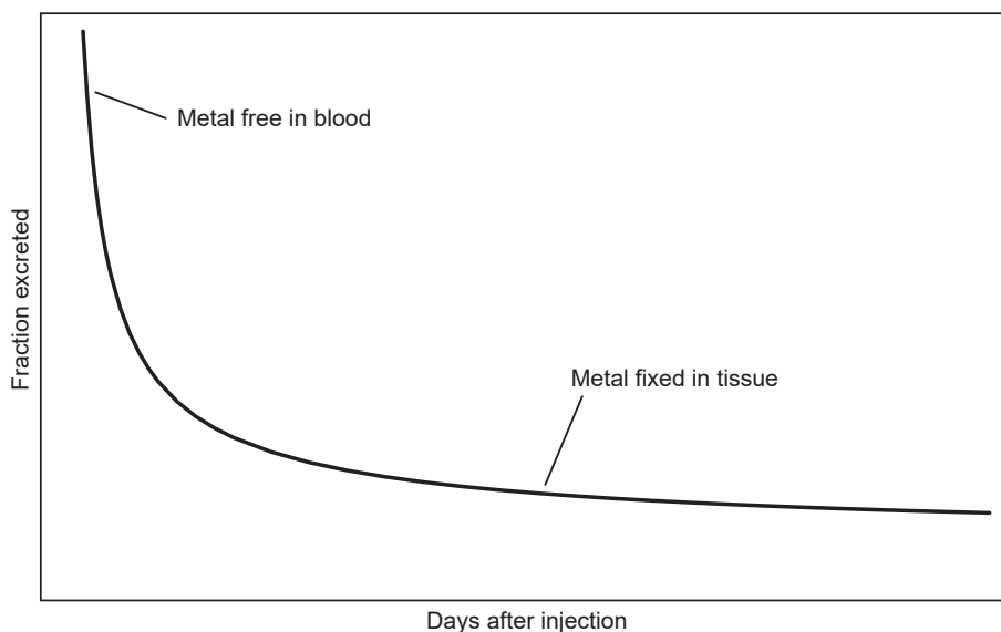
Figure 1. Daily Urinary Excretion for an Internal Exposure
